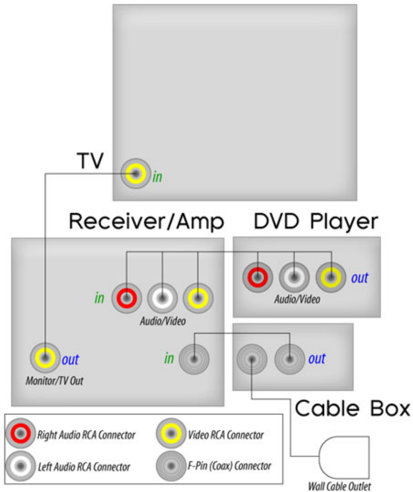
Diagram 1 illustrates a simple home theater configuration consisting of a TV, cable box, DVD player and a receiver/amp.
